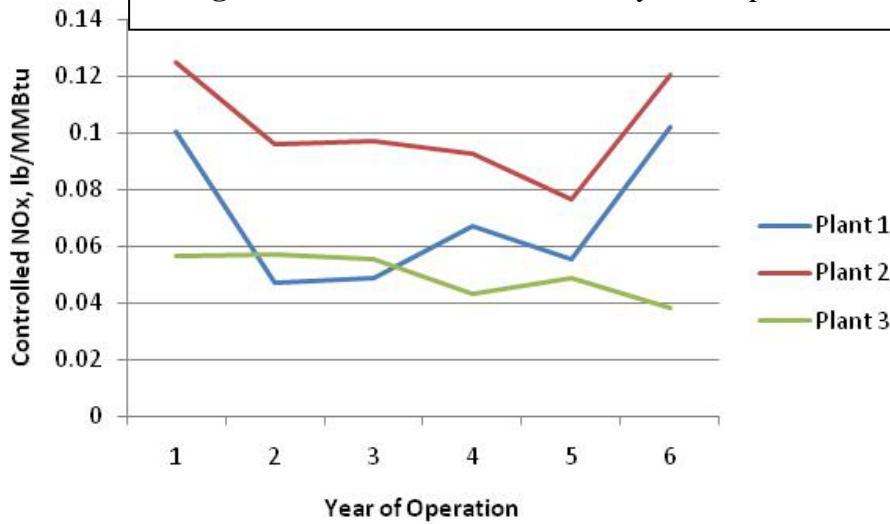
Figure 16. Controlled NOx versus year of operation
