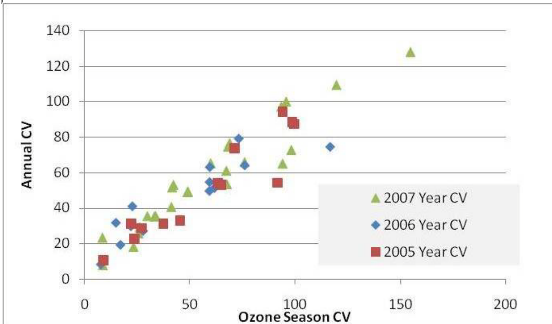
Figure 15. 2007 CV in Hourly NO x Emission rate for 25 annually controlled plants
