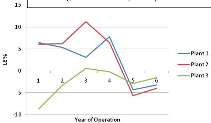
Figure 18. LE versus year of operation
