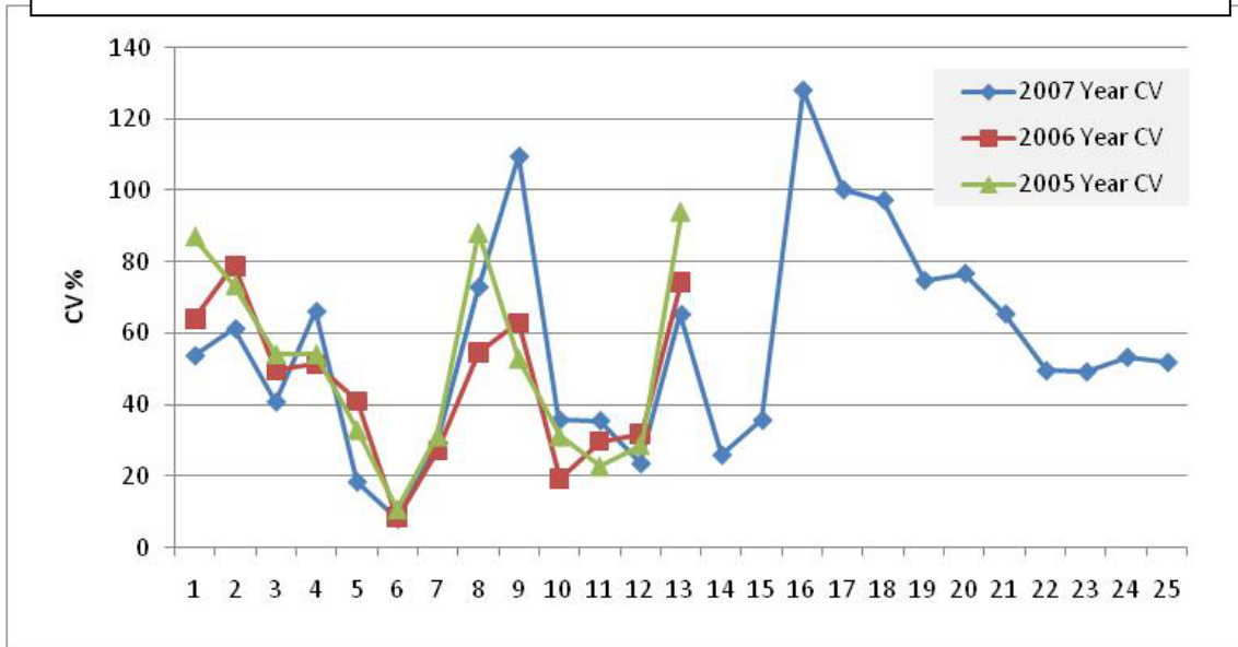
Figure 14. 2007 CV in Hourly NO x Emission rate for 25 annually controlled plants
