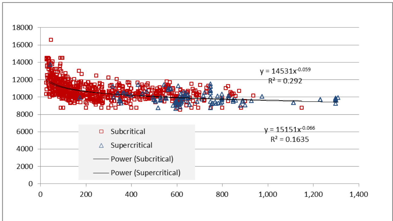
Figure 2. Plot of heat rate versus capacity for Subcritical and Supercritical boilers (NEEDS v4.10)
